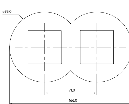
Ref. 43920 T - SV Duplo
