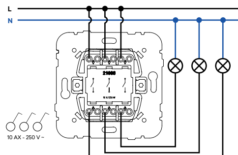
Triple Interruptor
